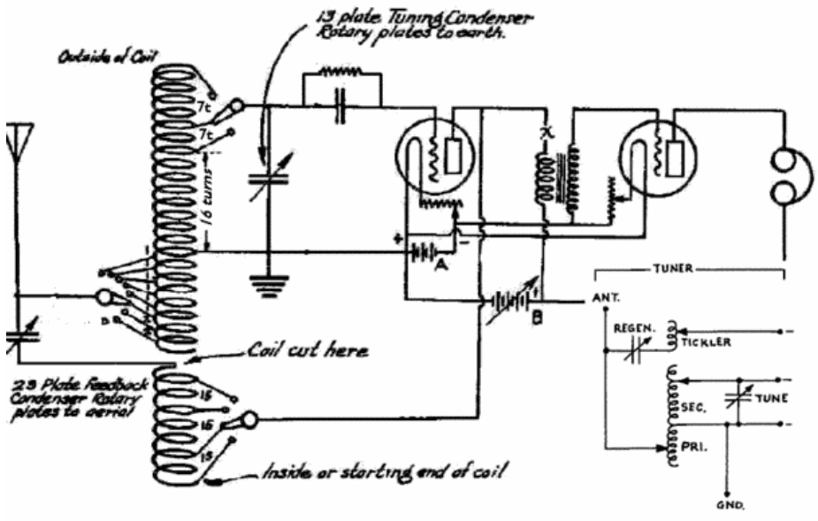
schema Reinartz tuner
